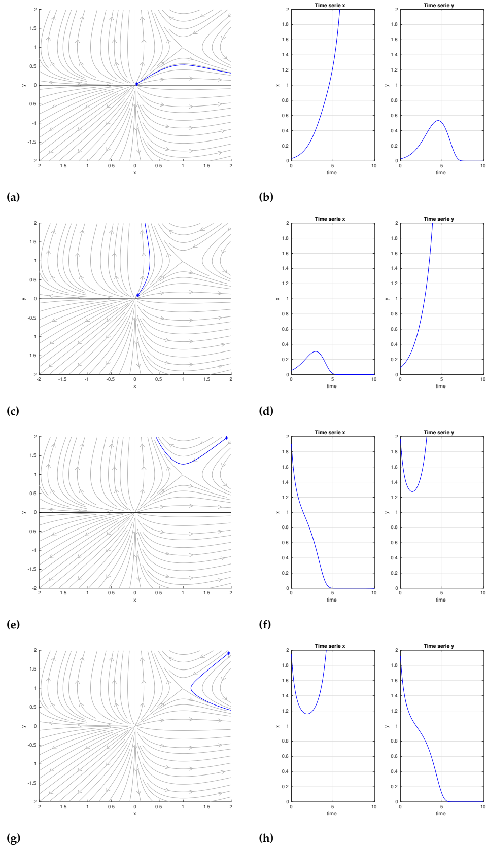
Figure 2. Case 1 simulations. This case occurs when vehicle entry rates are higher than exit rates in both categories. In (a,b), both technologies grow; however, finally, the conventional one dominates, while in (c,d), the opposite occurs. In (e,f), both technologies decrease, but the electric one manages to recover; while in (g,h), the opposite occurs.
